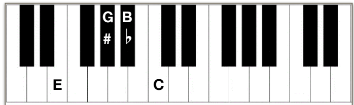
1st Inversion
