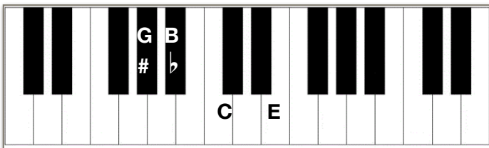
2nd Inversion
