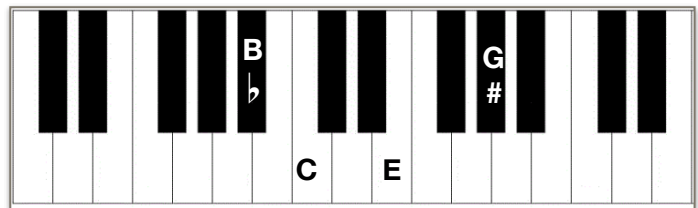
3rd Inversion
